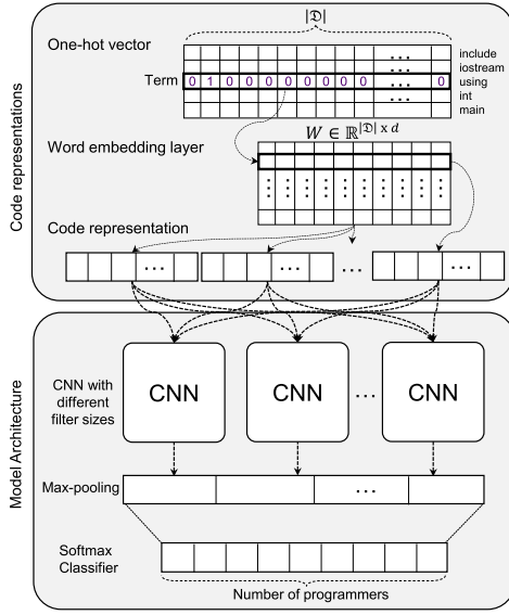
Fig. 1. C-CNN architecture with word embedding layer. The CNN model include multiple convolutional layers with different filter sizes.
