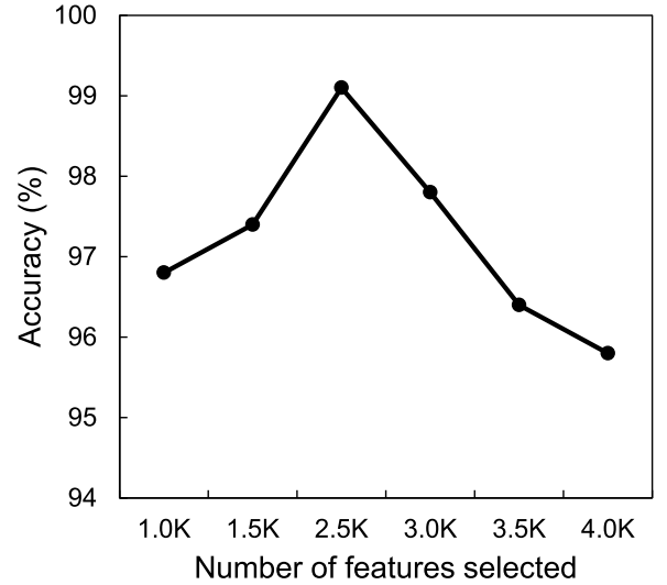
Fig. 5. Accuracy as the number of features of TF-IDF increased.
