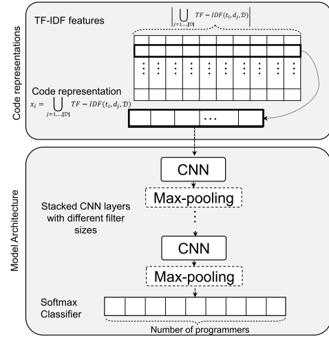
Fig. 3. S-CNN architecture with TFIDF representation. The CNN model stacks multiple convolutional layers with different filter sizes.
