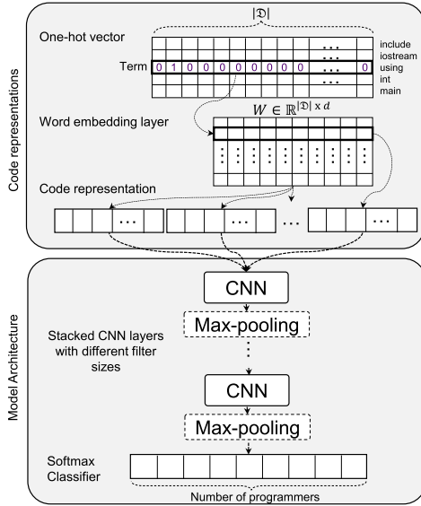
Fig. 2. S-CNN architecture with word embedding layer. The CNN model stacks multiple convolutional layers with different filter sizes.
