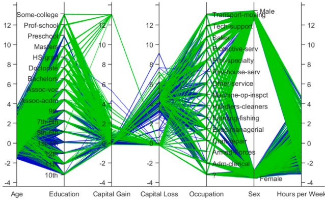
Fig. 7. PCP: The UCI Census training data is presented in a single graph to reveal a 2D pattern. The z-score on the y-axis is plotted against each feature value. The graph can aid in deciphering feature correlations and identifying helpful predictors for class separation. It can be seen in the distinct cluster, the features of age and education have a significant role in determining a given class. In the class prediction, the capital gain, on the other hand, does not create separation boundaries. Thus, this feature may be left out of the classification task. The green line represents the target value > 50K, and the blue line denotes income value < 50K.
