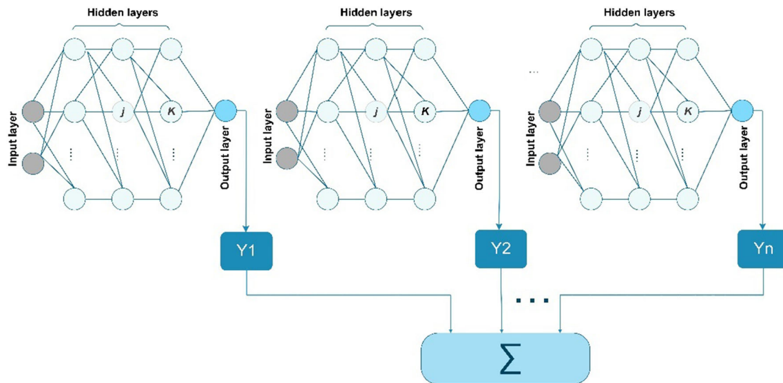
Fig. 4 Ensemble neural network
