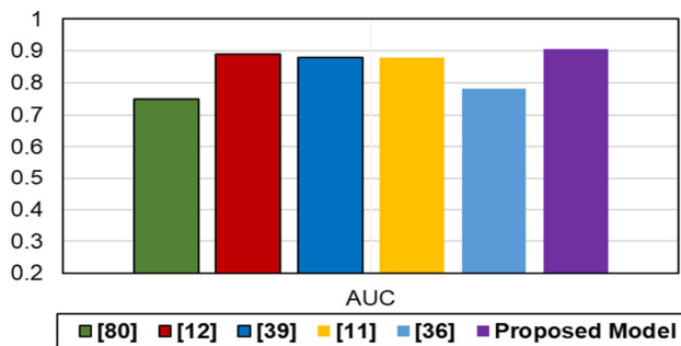
Fig. 13 Comparison with other models from the literature
