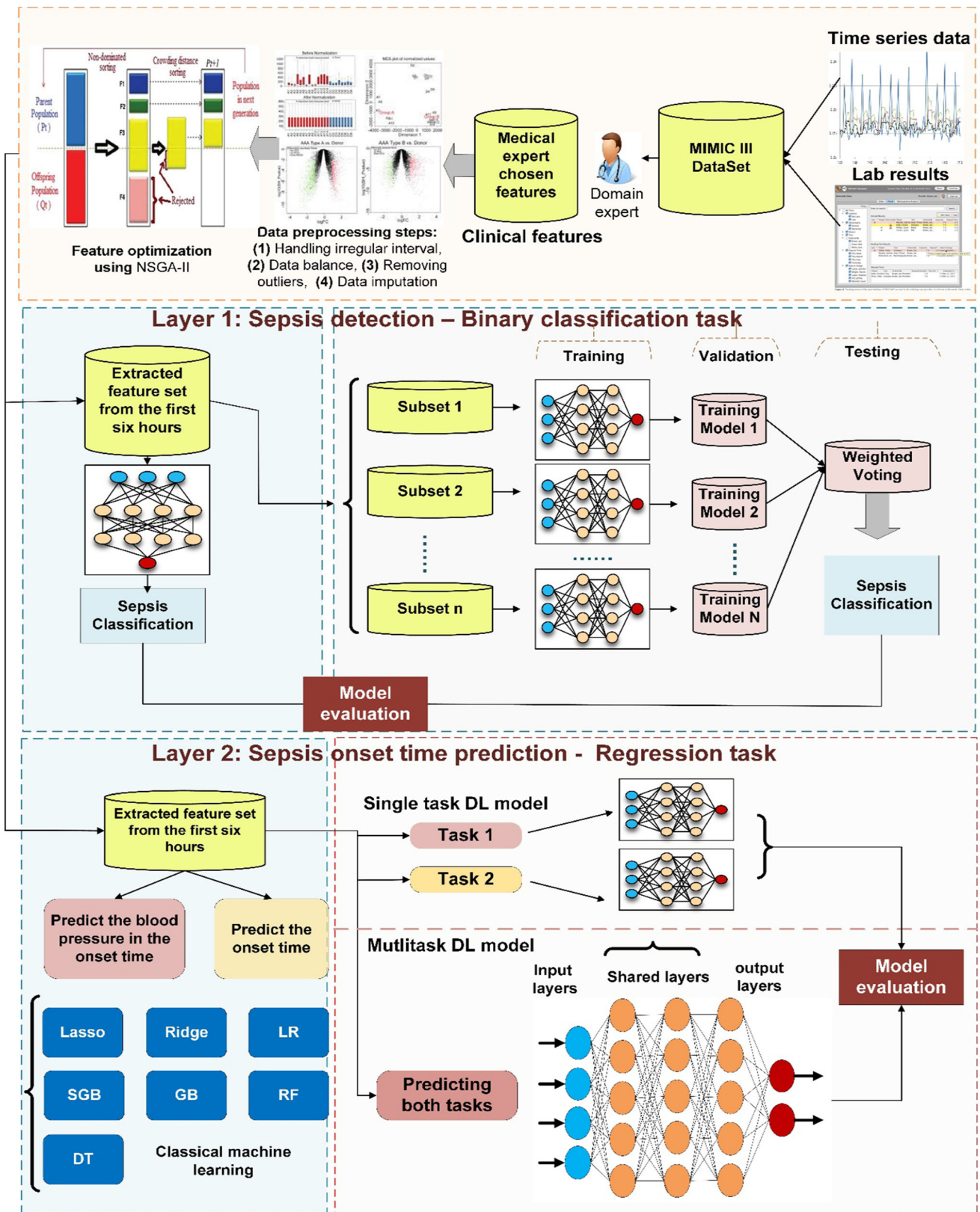
Fig. 5 The proposed framework
