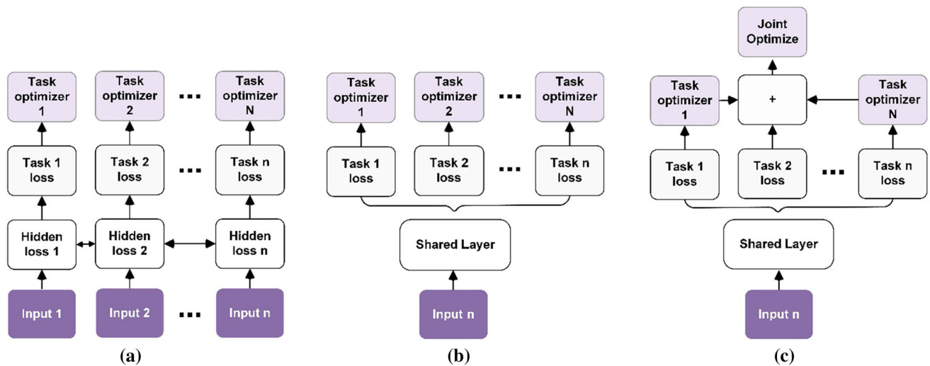
Fig. 1 Multitask architecture models: (a) Soft training: where each task has its own parameters and model, this is distance regularized to encourage distances to be similar, (b) Alternate training: this model
