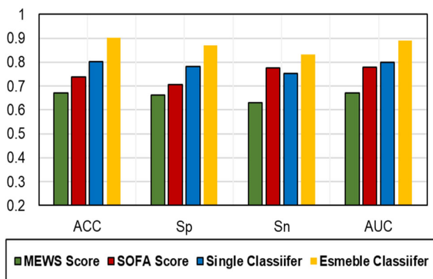
Fig. 11 Comparison with scoring systems
