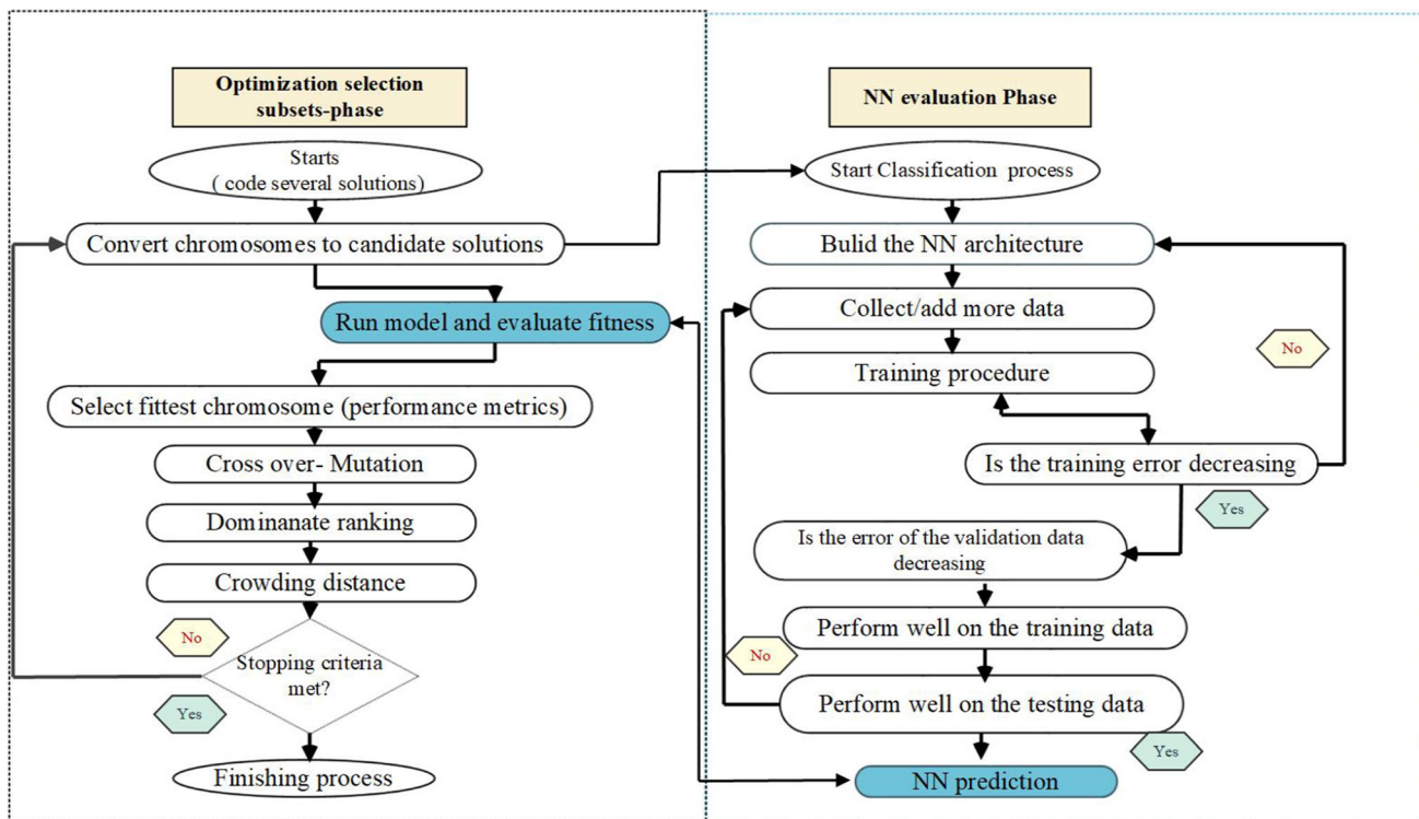
Fig. 8 Hybrid NSGA-II and neural network
